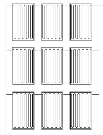
In parallel (Tichelmann method)
